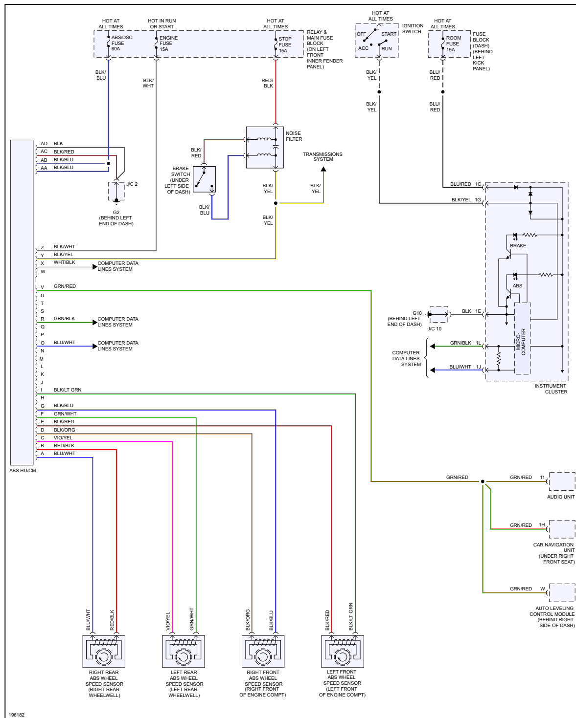
Fig 3: Anti-lock Brakes Circuit, W/O Dynamic Stability Control
